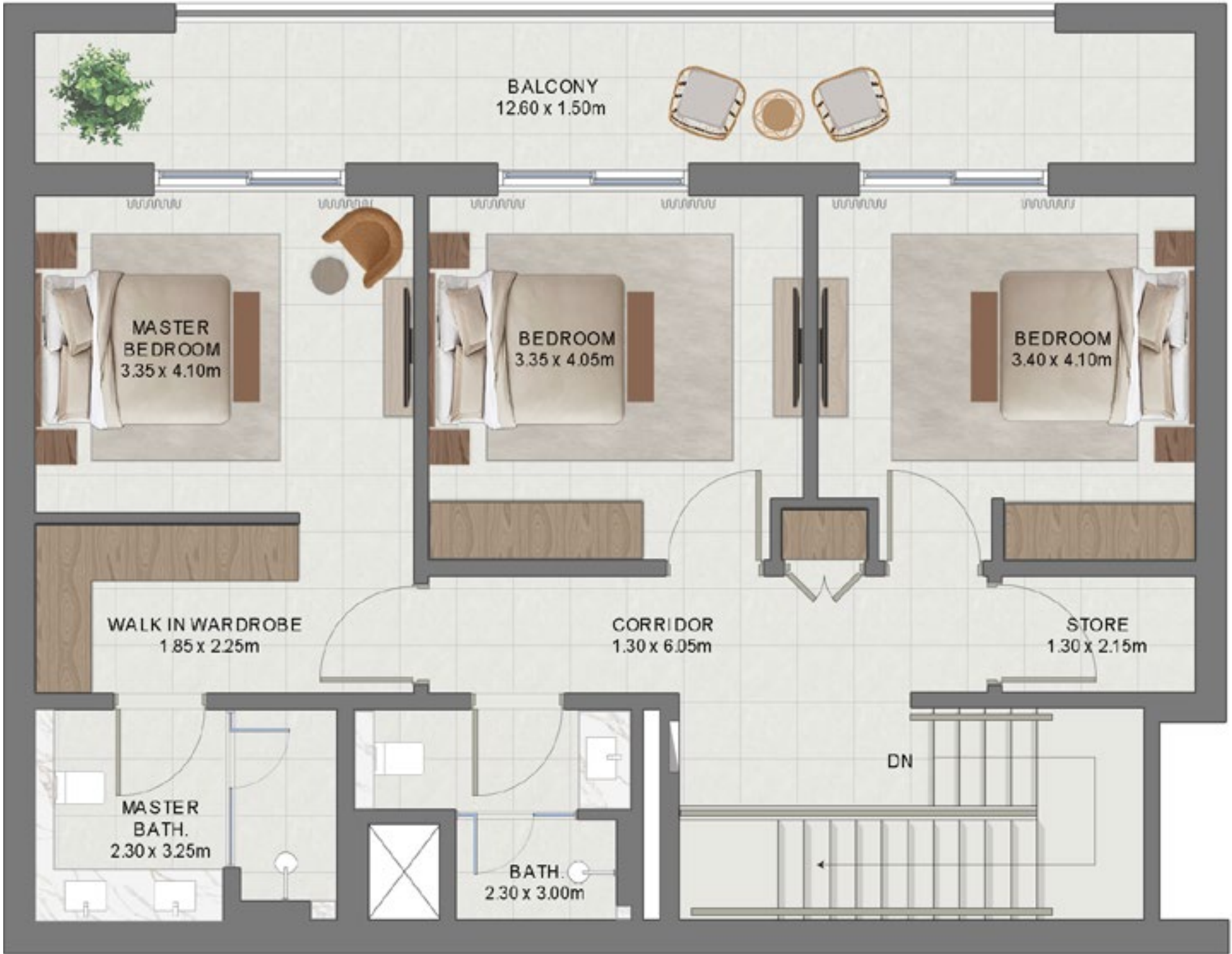
UPPER LEVEL
