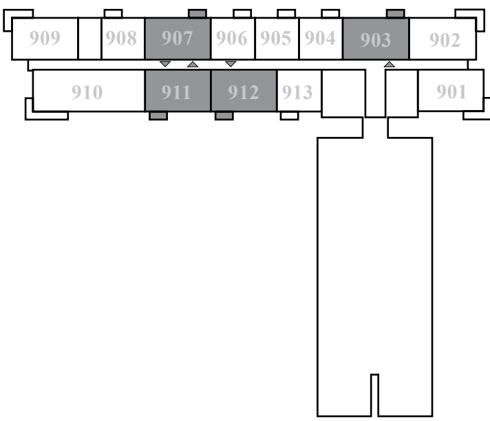
FLOOR 9-10
