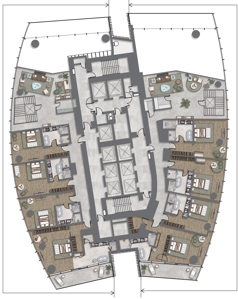
UPPER LEVEL 112
