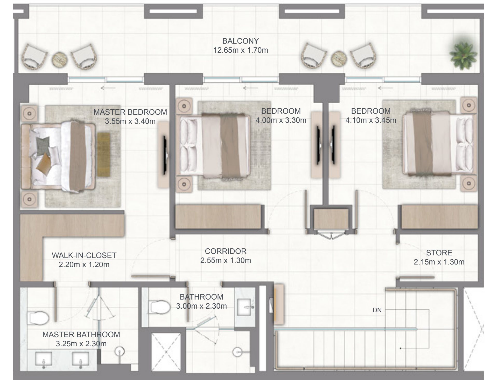
UPPER FLOOR
