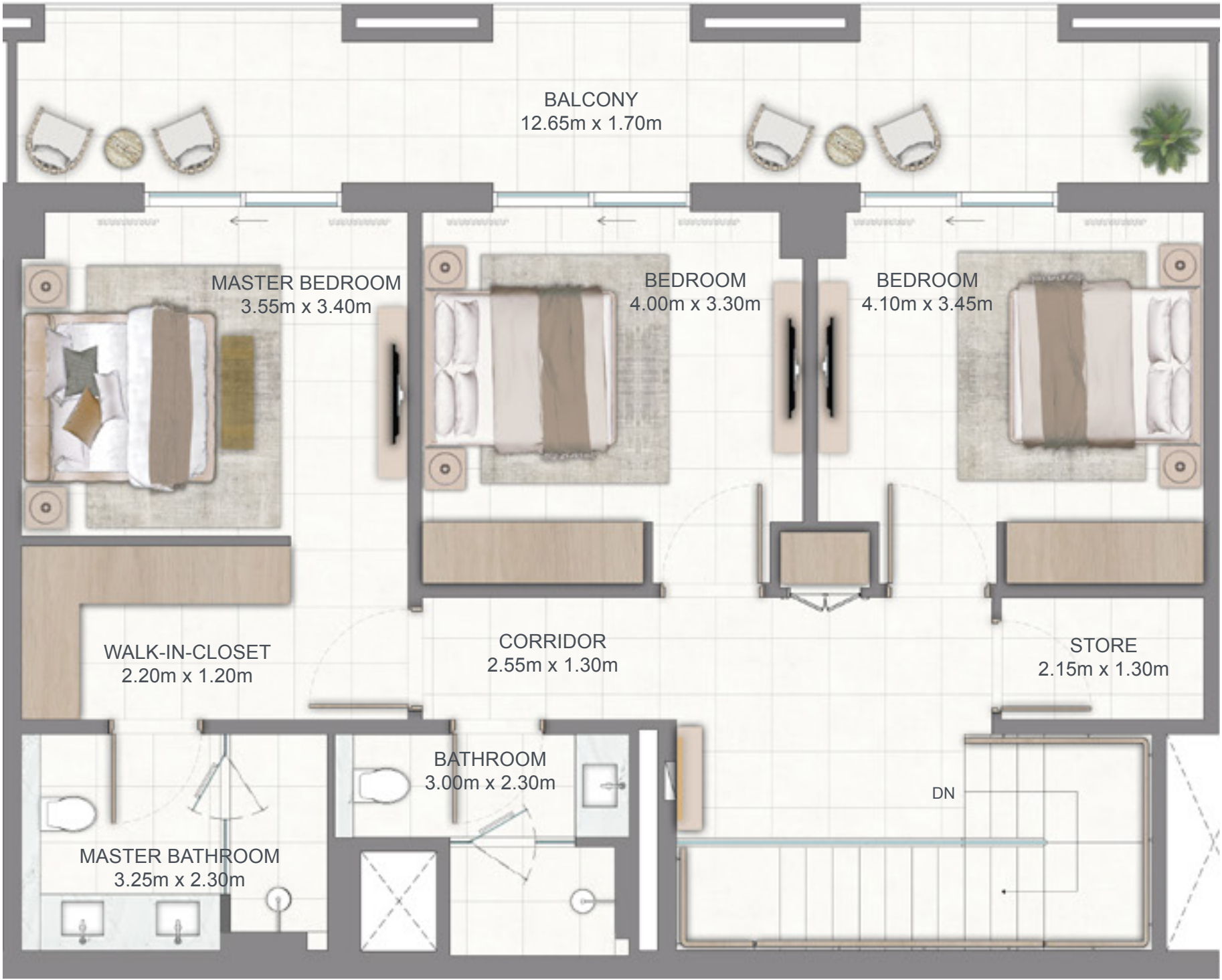
UPPER FLOOR
